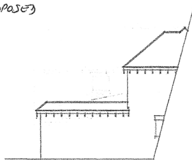
PROPOSED PART SIDE ELEVATION (facing due north) SCALE 1:100
